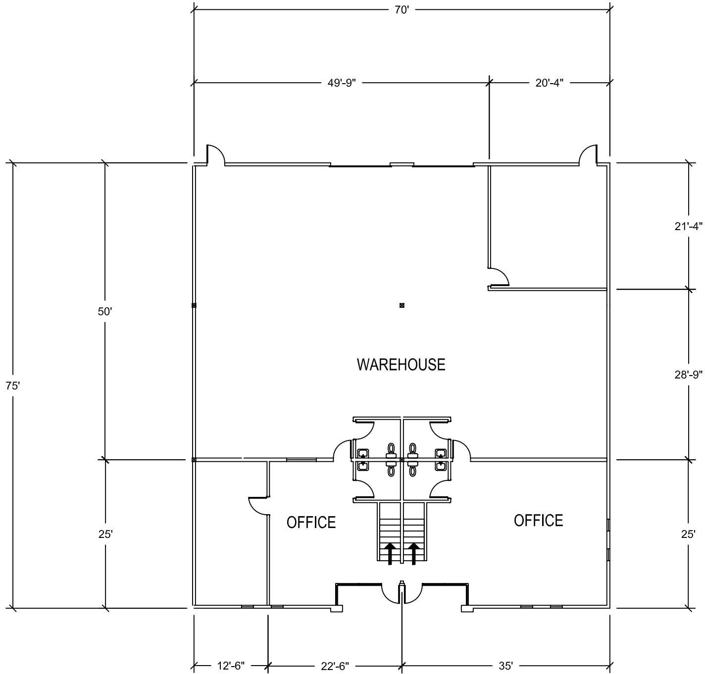
FIRST FLOOR
