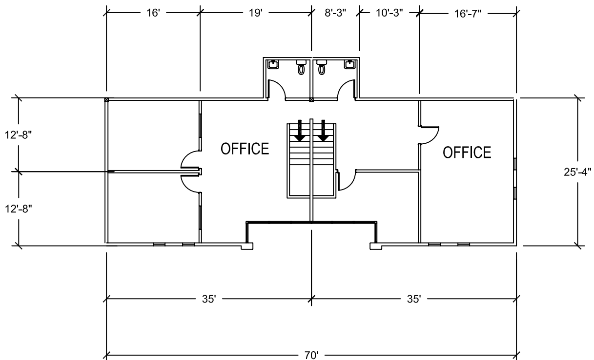
SECOND FLOOR
