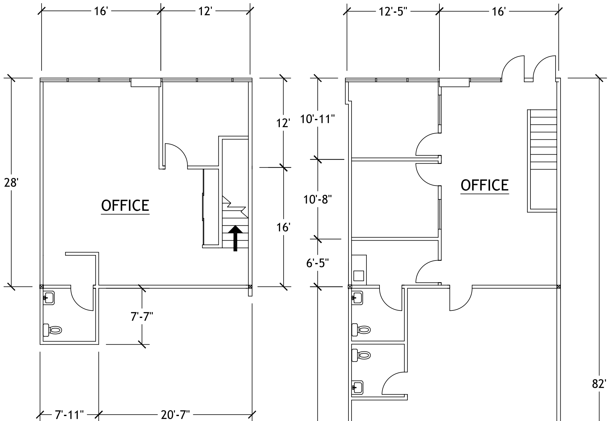
SECOND FLOOR
