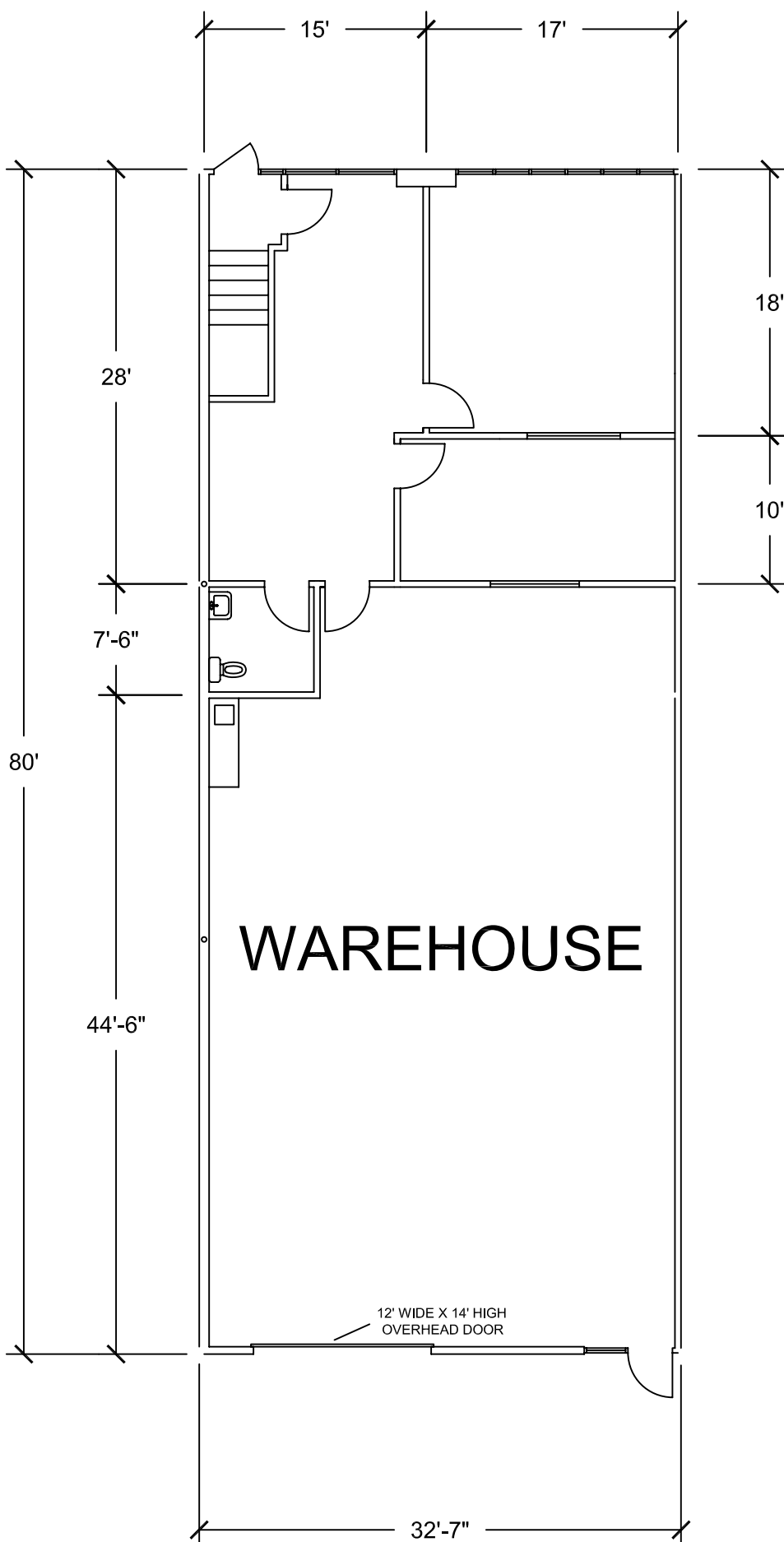
FIRST FLOOR
