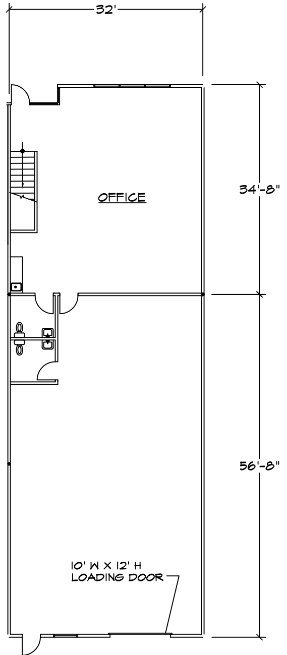
FIRST FLOOR
