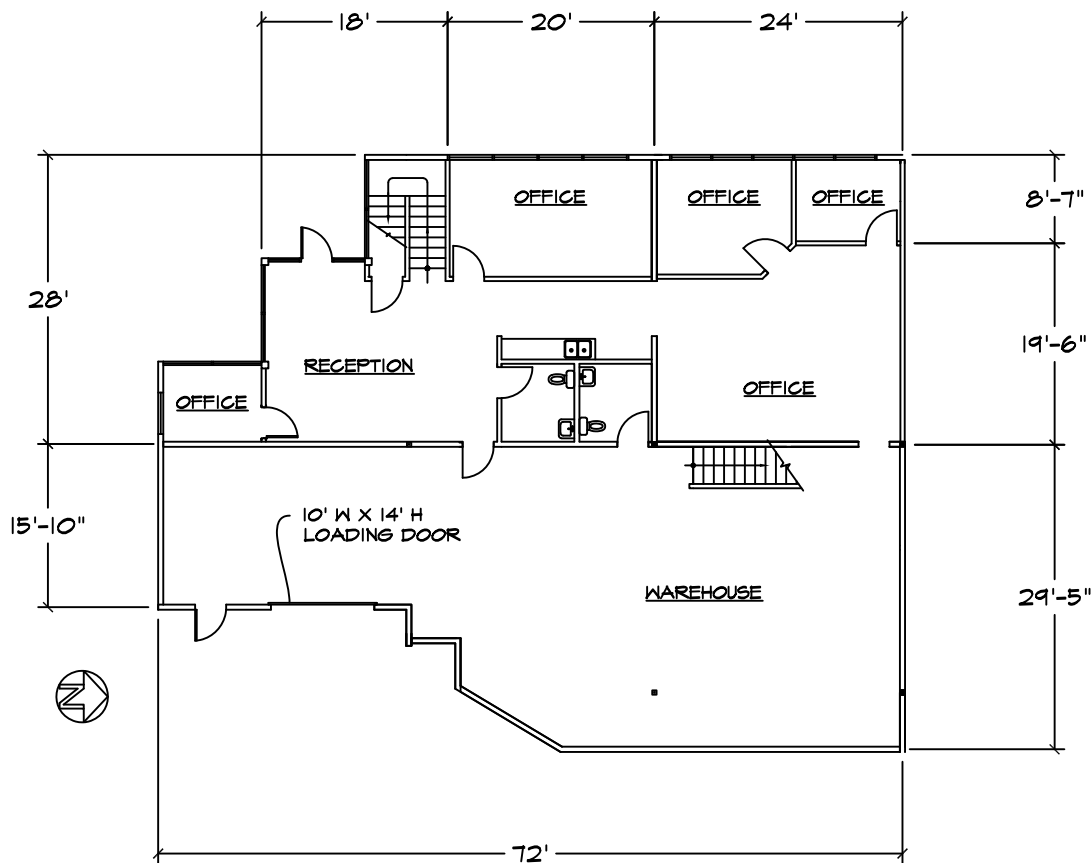
FIRST FLOOR
