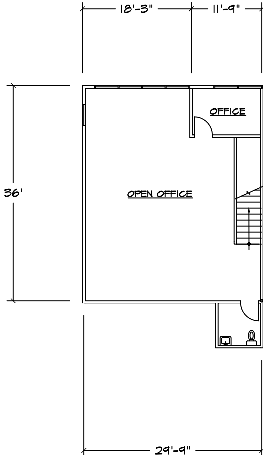
SECOND FLOOR
