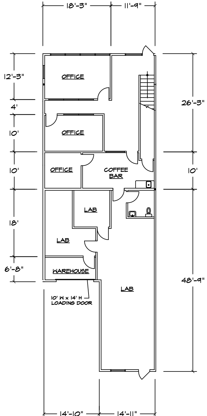
FIRST FLOOR
