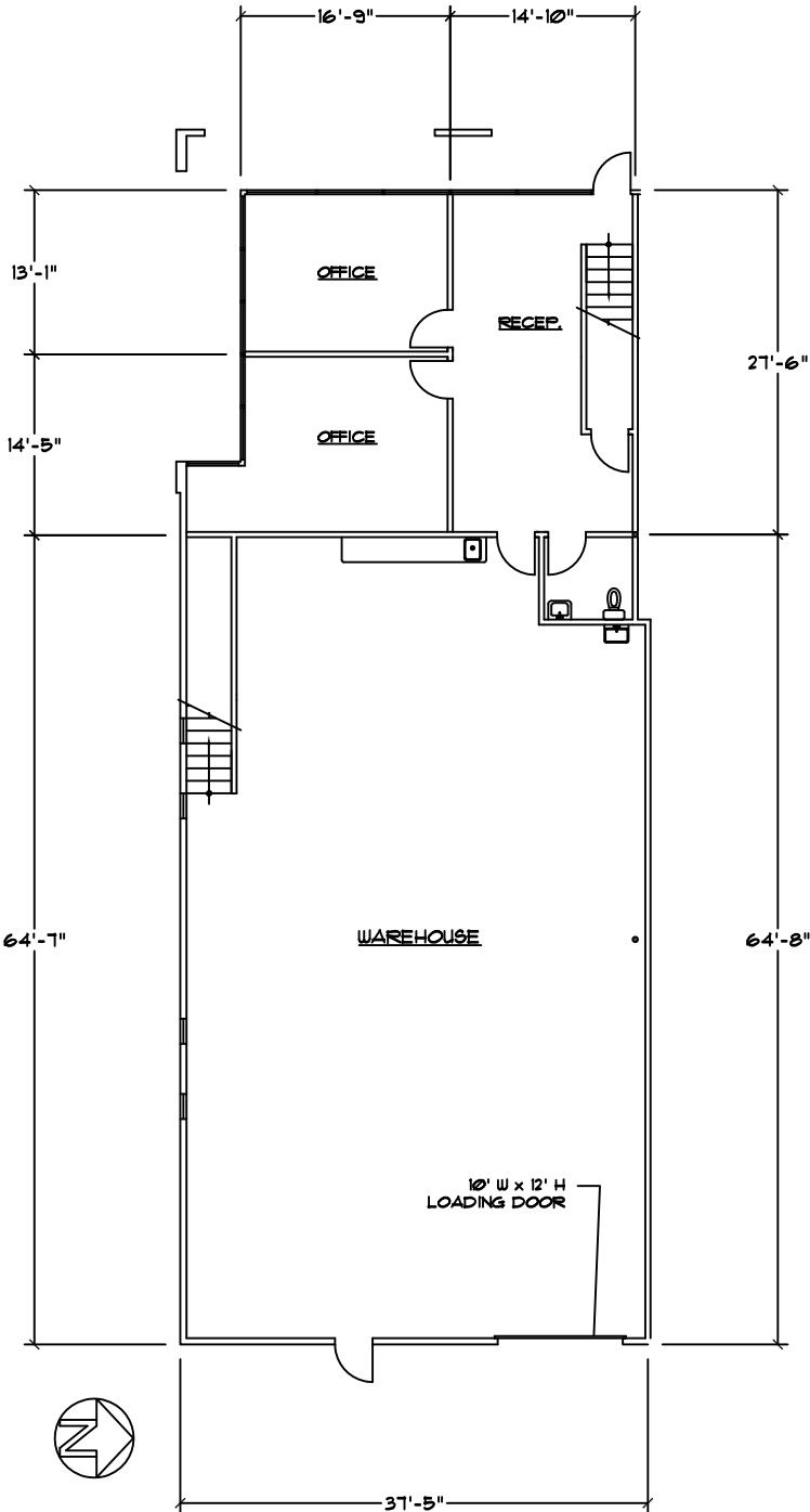
FIRST FLOOR
